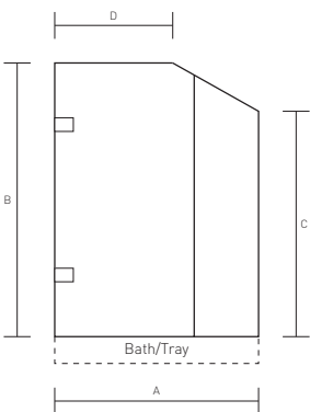
Diagram 6 - Corner Angle with Inline Panel (Left handed)
