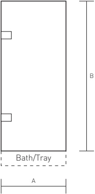
Diagram 4 - Door with 2 Inline Panels
