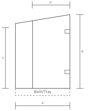
Diagram 13 - Corner Angle with Inline Panel (Right handed)
