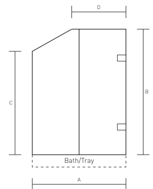
Diagram 9 - Corner Angle with Inline Panel (Right handed)
