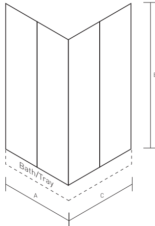
Diagram 8 - Bathguard
