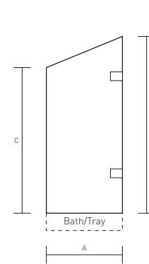
Diagram 5 - Complete Angle (Right handed)
