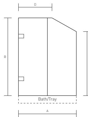
Diagram 8 - Corner Angle with Inline Panel (Left handed)
