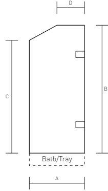
Diagram 3 - Corner Angle (Right handed)
