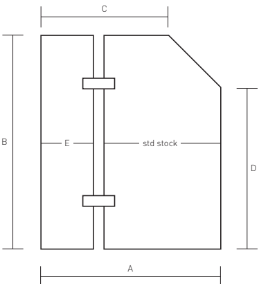
Diagram 6 - Standard Inline and Angle Door
