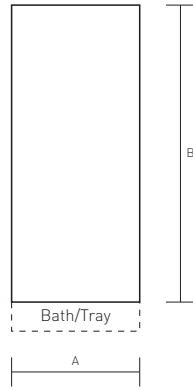
Diagram 5 - Corner Entry
