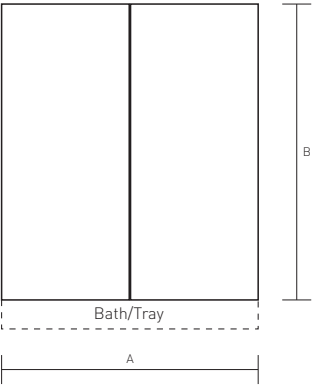
Diagram 8 - Angle Bath Screen
